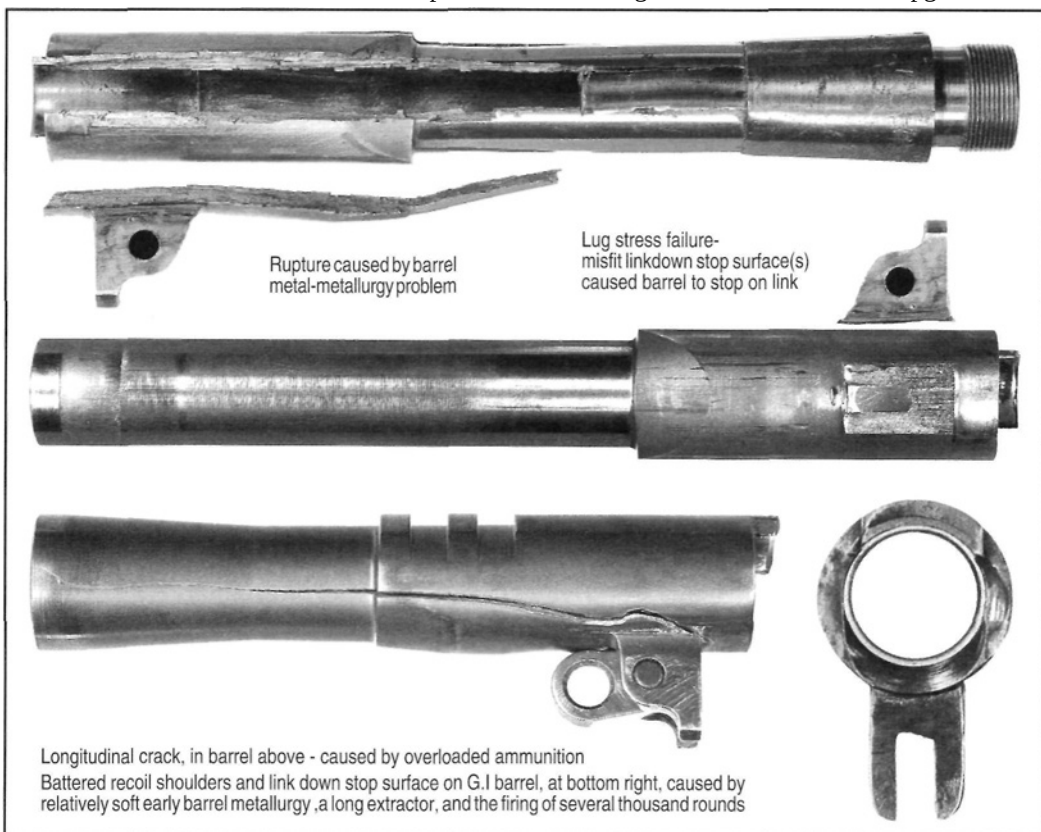
Figure 87- Shows views of defective/damaged commercial M1911 type barrels at top, center, and bottom. An unserviceable early U.S.G.I. M1911 barrel (rear view) is shown at bottom right. Battering peened the recoil surface into the chamber on the right side of this barrel and prevented case extraction.
