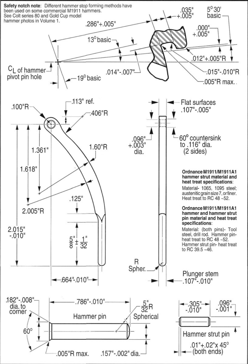
Figure 152- Ordnance style detail illustrations by Heritage - VSP staff artist show M1911/M1911A1 hammer safety notch, hammer strut, hammer strut pin, and hammer pin (pivot pin) dimensional inspection data. For further data see ordnance drawings #7790803 (NM hammer); #5503839 (std. hammer); #6008600 (hammer strut); #5013206 (hammer pin); and #5013207 (hammer strut pin).
