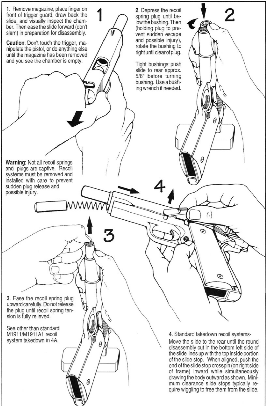
Figure 49- Ordnance style illustrations show M1911/M1911A1 Pistol disassembly steps 1 through 4.
