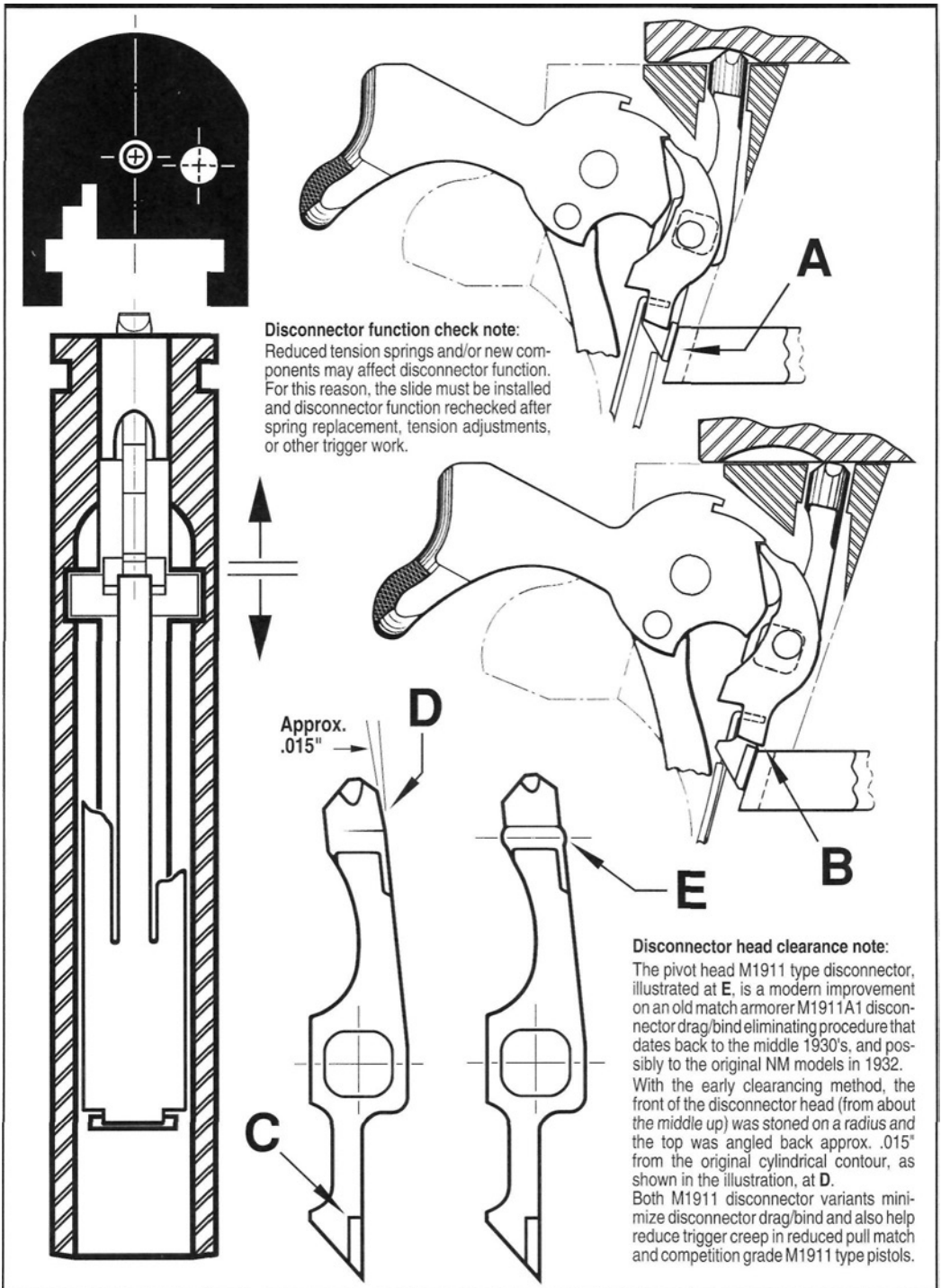
Figure 162- Ordnance style rear sectional illustration by Heritage - VSP staff artist, at left, depicts M1911A1 trigger group components installed in the frame for a final disconnecter function check with the slide after completion of trigger work. Disconnecter function checks (and rechecks) are particularly important when reduced tension and/or tuned springs are installed. Illustrations, at upper right, show an M1911A1 disconnecter in the trigger forward/connected and trigger rearward/disconnected positions. Steps that help eliminate disconnecter drag/bind, indicated at arrows above are: (1) polish the backs of the disconnecter and trigger bow, at A ; (2) lightly edge break or radius the sear hooks and disconnecter blade corners (up to a max. of .003") at B and C ; and (3) disconnecter head clearance. See note, above.
