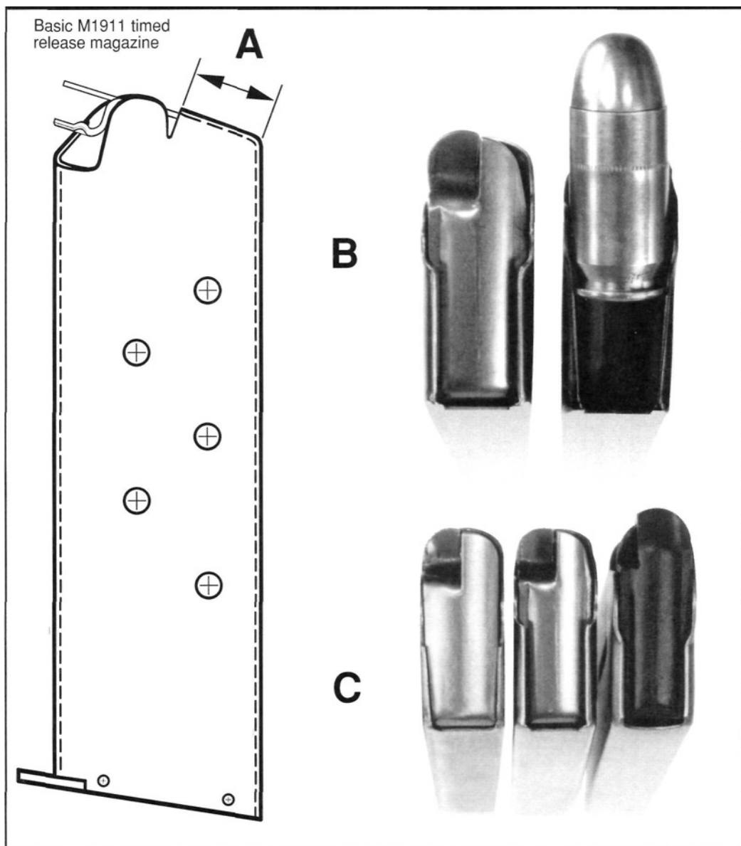
Figure 170- Ordnance style illustration by Heritage - VSP staff artist shows one of several magazine feed lip modifications historically employed to control and time cartridge release in M1911 type magazines. Although several variations exist, dimension A , in most magazines modified as illustrated in the above example, typically measures between .55" and .60". Cartridge release in ordnance std. dimension M1911A1 magazines depends primarily on feed lip width and cartridge rim diameter. The photo, at B , shows top views of a timed release and standard magazine for comparison. The max. rim diameter cartridge in the standard magazine releases when pushed forward to a point approx, even with the release slots in the timed release magazine next to it. A minimum rim diameter cartridge in the same magazine, however, releases fractionally earlier, i.e., forward of the cartridge position shown. Top views of several commercial timed release M1911 magazines are shown below, at C , for comparison. Considering the quality of currently available name brand timed release M1911 magazines, it's no longer worthwhile to invest time in modifying and tuning ordnance standard magazines. Timed release magazines are less cartridge rim diameter and rim condition sensitive, and as the name implies, mechanically time release and thereby control cartridge horizontal breakover and chamber alignment. Historical note: The first timed release M1911 magazines were ordnance std. dimension magazines modified by service marksmanship unit armorers to improve ramping and chambering of match cartridges (notably wadcutter type) in NM pistols. Magazines were then custom fit for best function in specific pistols.
