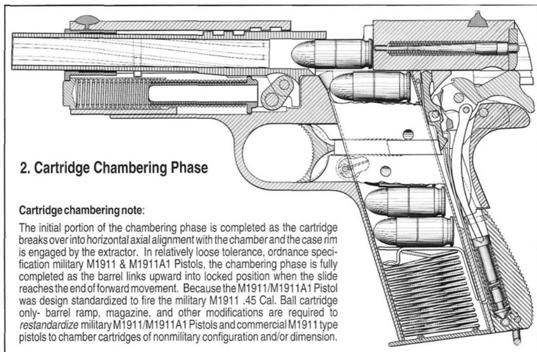
Figure 26- Ordnance style sectional illustration by Heritage - VSP staff artist shows relative positions of components in an M1911 type pistol at the beginning of the cartridge chambering phase. Chambering occurs when a round is fed from the magazine, as shown above, and placed in the chamber. This function takes place as the slide assembly moves forward under pressure of the compressed recoil spring, strips a cartridge from the magazine, and then pushes the cartridge up the barrel ramp and into the chamber.
