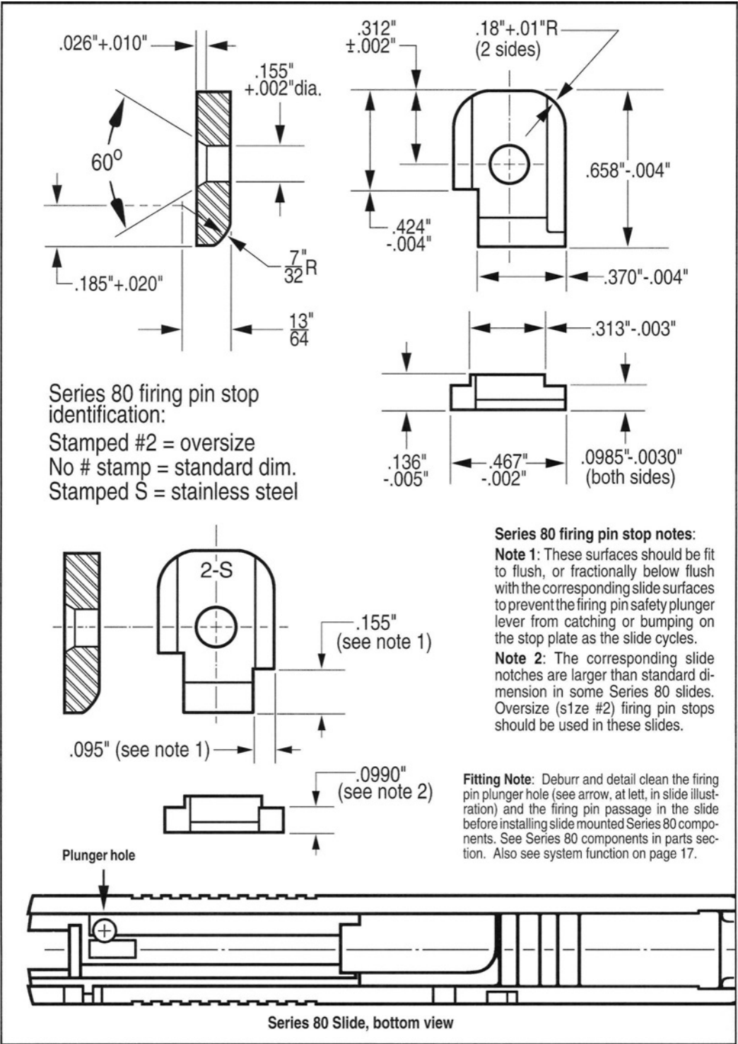
Figure 130- Ordnance style drawing by Heritage - VSP staff artist, at top, shows M1911/M1911A1 firing pin stop plate dimensional inspection details. Series 80 dimensional differences are shown and discussed below. Ordnance specified M1911A1 and M1911A1 NM firing pin stop material and heat treat: material- 4140 or 4150 steel, austenitic grain size 6 or smaller; heat treat to RC 43.5 to 50. For further data, see ord. drawing #5013205. Loose firing pin stop plate fit remedies: (1) trial fit and install an oversize plate, or (2) tighten fit by 3 point dimpling the outer edges of the plate with a prick punch.
