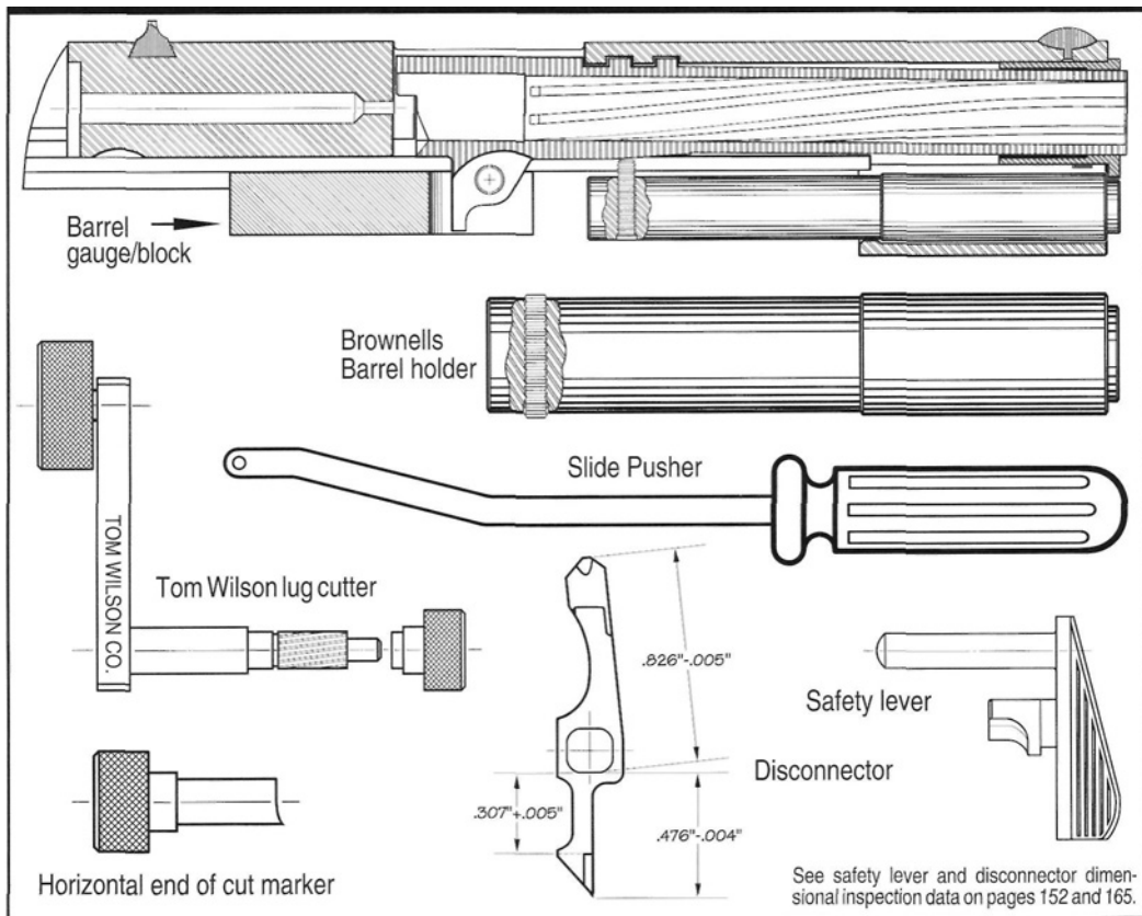
Figure 119- Sectional illustration by Heritage - VSP staff artist, at top, shows a Brownells barrel holder installed in an M1911A1 slide in preparation for bottom barrel lug cutting. The barrel gauge block shown is temporarily installed to align the bottom lug before tightening the barrel holder. Tooling illustrated, except for the gunsmith made end of cut marker, is available from Brownells, Inc. A serviceable disconnecter, safety lever, and rear spring are also useful fit check and fitting tools.
