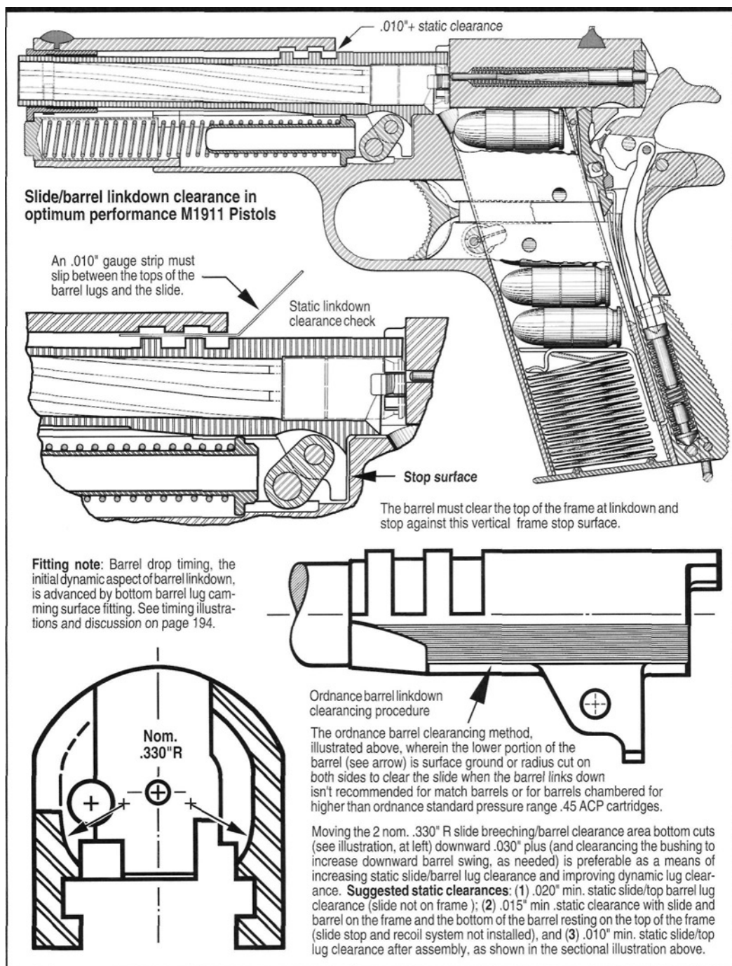
Figure 178- Ordnance style sectional illustration by Heritage - VSP staff artist, at top, shows suggested slide/barrel lug static clearance in an assembled optimum performance M1911 Pistol. Interior slide clearing to improve static and dynamic slide/barrel lug clearance at link down is shown below. Two basic lug clearance conditions must be met: (1) Static- the barrel must link down and stop against the frame's vertical stop surface- and link down far enough to allow the slide to clear the barrel lugs. (2) Dynamic - the barrel must be able to link down fast enough from the vertical + horizontal lug engaged position to permit the slide to clear the corners of the top barrel lugs on recoil. Dynamic requirements: (1) faster link down timing (one reason for combining a mid vert, stack slide, a .302" lug barrel, and a shorter link); (2) eliminate link down interference by clearing as above and on page 194; and (3) retard initial slide movement as much as possible. Also see barrel-slide-frame fitting for optimum reliability on page 195.
