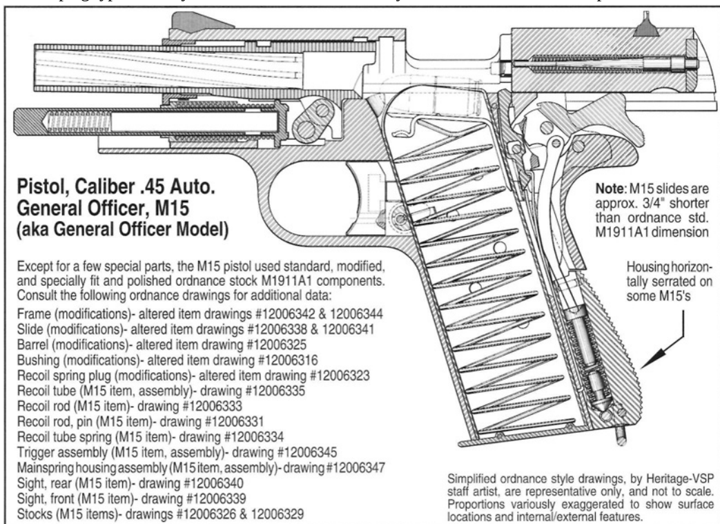
Figure 124- Ordnance style sectional illustration by Heritage - VSP staff artist shows an interior view of an M15 General Officer Pistol. M15 components are listed above. Major differences shown on page 137.
