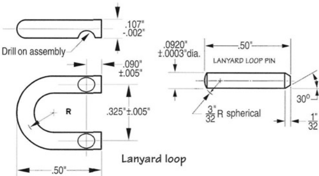
Figure 158- Ordinance style illustrations by Heritage - VSP staff artist show basic M1911/M1911A1 mainspring housing subassembly component dimensional inspection data. For further component data, see the above listed ordinance drawing numbers. Mainspring (hammer spring) dimensional inspection data and compression test data is shown in figure 157.
