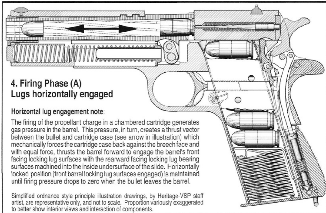
Figure 29- Sectional illustration by Heritage - VSP staff artist shows relative positions of components in an M1911A1 Pistol during the initial firing phase, when the bullet is still in the barrel. Firing occurs in an M1911 type pistol when the grip safety is depressed; the trigger is squeezed; and interaction of the trigger bow, disconnecter, and sear releases the hammer. The hammer then rotates forward and strikes the inertial firing pin which, in turn, initiates and ignites the primer in a chambered round. The barrel and slide remain locked firmly together (both horizontally and vertically) during the initial firing phase, as shown above.
