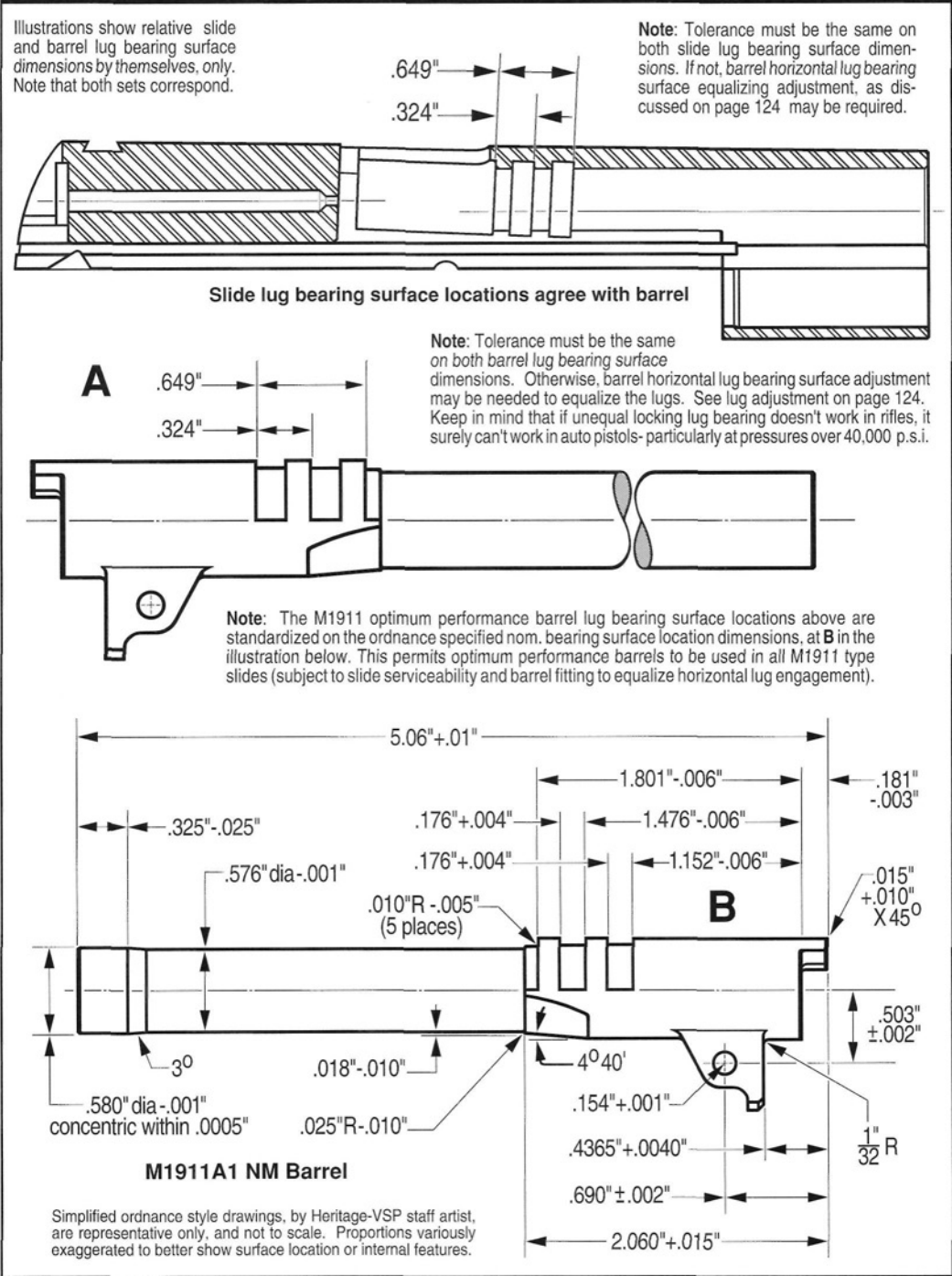
Figure 176- Ordnance style principle illustrations by Heritage - VSP staff artist, at top, show matching slide and barrel lug bearing surface locations proposed for optimum performance M1911 slides and barrels. Correspondingly equal slide/barrel lug bearing surface locations and equal tolerances on both the barrel and slide lug bearing surfaces permit all 3 slide and barrel lug bearing surfaces to bear uniformly in the horizontal plane (less a lug surface contact area deduct for barrel elevation angle). Relative optimum performance barrel lug bearing surface locations, at A , are the same as those shown in the NM barrel illustration at B , but in simplified form without dimensional reference to the recoil surfaces. Note: If lug bearing surfaces are not equal in higher than design pressure pistols, or at least close enough to effectively pressure seat without damaging the barrel, lug failures as shown on page 185 will sooner or later result.
