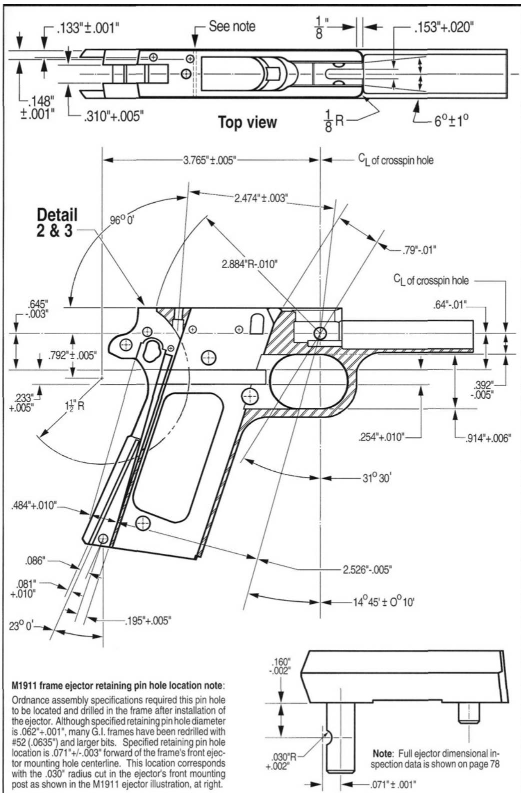
Figure 55- Ordnance style illustrations by Heritage - VSP staff artist show M1911/M1911A1 top frame and longitudinal sectional views with critical surface locations and dimensions.
