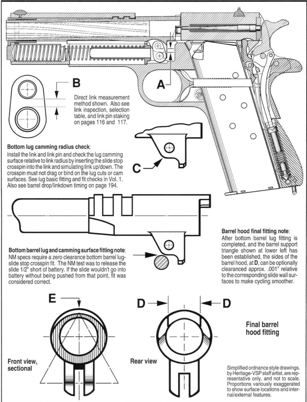
Figure 121- Arrows, at A, in the ordnance style sectional illustration, at top, indicate the vertical distance between the cut bottom barrel lug surface and the bottom of the barrel link pin hole. This critical distance, measured after removing the barrel, determines barrel link length. Specifically, the link selected must have the same pin bearing surface spacing, as referenced at B. Although identified by hole center location, barrel links should be selected with a digital caliper based on actual hole space measurement only. The illustration below shows the lug cam area, at C, radiused (best tool is an Eze-Lap diamond hone) to facilitate barrel link up/cam up and link down. Illustrations at bottom show the sides of the barrel hood, at D, that are final cleared after the bottom lug is cut and the barrel is triangularly supported in locked position. If best link size is slightly tall, (vertical lock too tight) and the next shorter link size binds the slide stop crosspin, fine adjust the rear barrel lug slot bottom, at E, to fractionally raise vertical lug contact.
