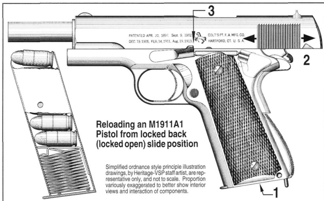
Figure 38- Sectional illustration by Heritage - VSP staff artist shows relative positions of components relative to slide stop position in a standard, ordnance spec. M1911A1 Pistol with the slide in locked position. Placing a loaded magazine in the pistol, at 1 , drawing the locked slide rearward, at 2 , to disengage the slide stop, at 3 (or thumb depressing the slide stop to release the slide) strips and chambers the first round from the loaded magazine and brings the operating cycle full circle. See Phase 1 on pg. 40.
