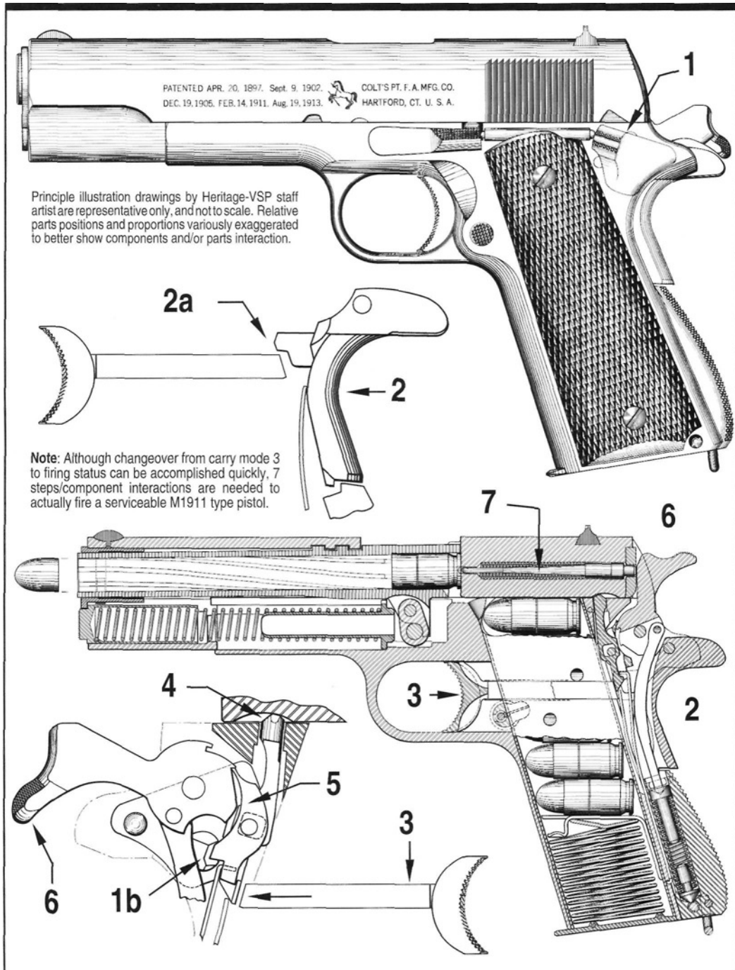
Figure 23- Illustrations show the mechanical steps/functions required to change the status of an M1911 type pistol from cocked and locked condition, to ready to fire , to firing mode - and the sequence of component interactions that must occur. The thumb safety is moved to the ready position, at 1, in order to rotate the sear stop (1b) and thereby unblock the sear. The grip safety, at 2, must be depressed to elevate the trigger stop (2a) to permit rearward movement of the trigger, at 3. With the slide forward and the disconnector connected as shown at 4, squeezing the trigger (3) applies pressure to the disconnector, causing it to rotate the sear, at 5. This action releases the hammer, at 6. The hammer (6) then strikes the inertial firing pin (7) which, in turn, fires the chambered round. This sequence can occur only as the result of deliberate action- hence the ordnance truism that serviceable M191/M1911A1 Pistols have to be intentionally fired. Carry Mode 3 was used by the military in combat and security enforcement zones.
