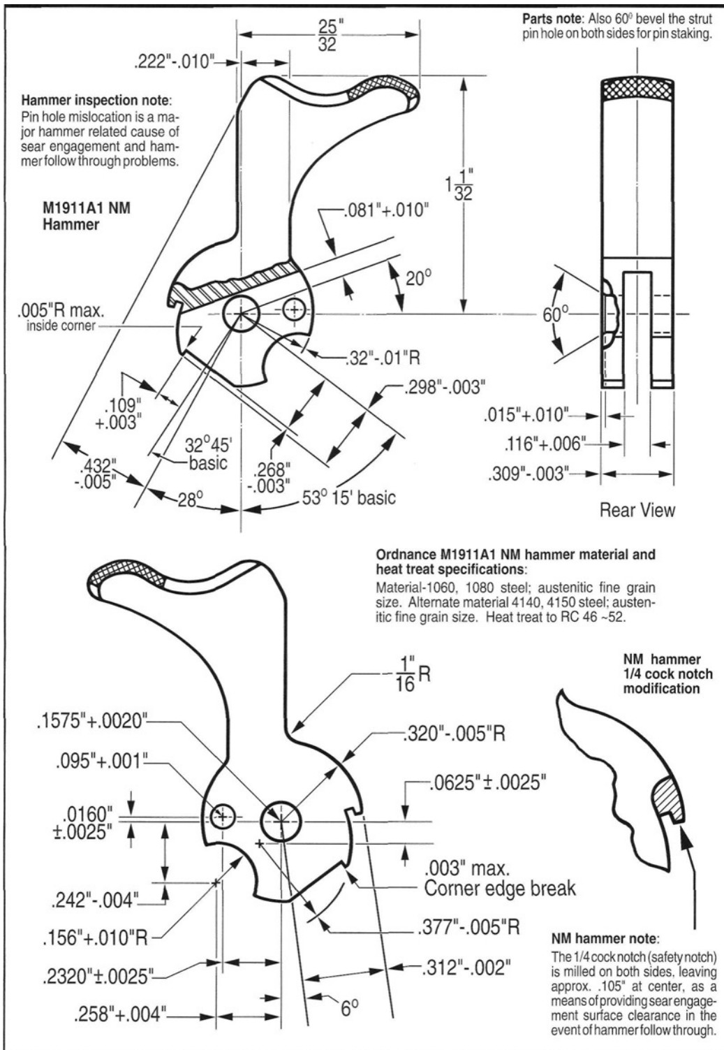
Figure 151- Ordinance style illustrations by Heritage - VSP staff artist show M1911A1 NM hammer dimensional inspection details. 1/4 cock mod. shown at lower right. Note 1: The non pinch variation of the 7/16" wide spur M1 911 hammer was still specified as an acceptable production alternative at time of publication. Note 2: Both 45° diamond cut (std.) and straight crosscut (alt.) hammer spur knurling patterns are still specified. For further data see ord. drawings #7790803 (NM hammer) and #5503839 (std. hammer).
