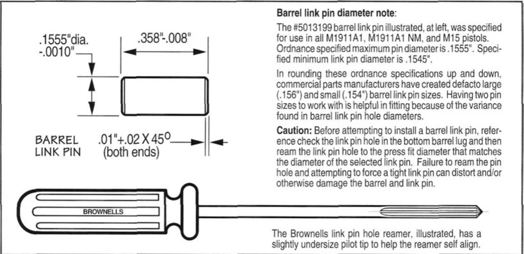
Figure 104- Ordnance style illustration by Heritage - VSP staff artist, at top, shows M1911/M1911A1 and M1911A1 NM barrel link pin dimensional inspection data. Ordnance link pin material/hardness specifications are: tool steel drill rod, heat treated to RC 43.5 to 50 before grinding to specified diameter. A Nowlin link pin hole reamer, available from Brownells, Inc., is shown, at bottom. Link pin reamers are available in nom. .154" and .156" diameter sizes.
