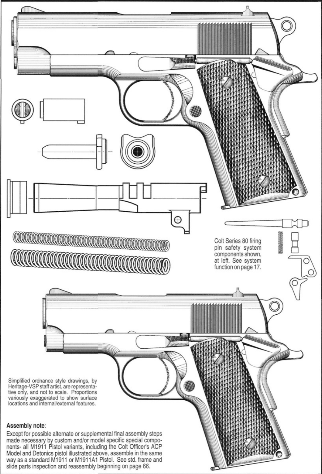
Figure 127- Ordnance style illustration by Heritage - VSP staff artist, at top, shows Colt Officer's ACP Model component differences which include an approx. 3 1/2" barrel; a short cone type barrel bushing; dual/concentric recoil springs; an extra short recoil spring guide, and a short recoil spring plug with slide locking tab. An ultra short early Detonics M1911 variant is illustrated below for comparison.
