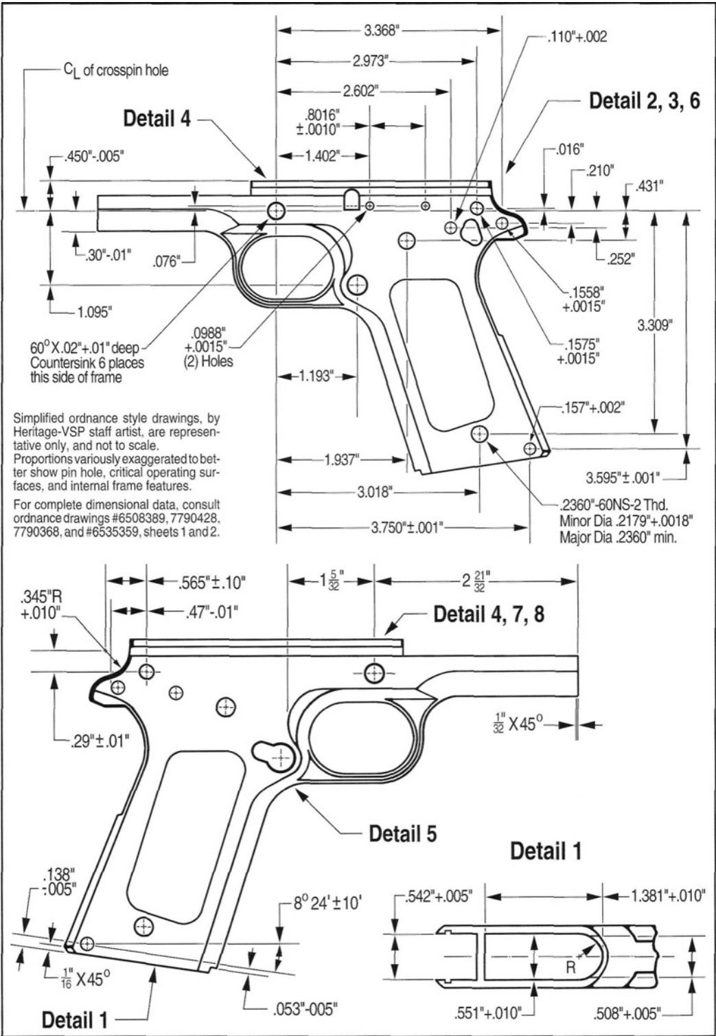
Figure 54- Illustrations by Heritage - VSP staff artist show M1911/M1911A1 frame views and critical operating surface locations and dimensions. Enlarged surface/area detail views, included above and on the following pages, provide additional component dimensional inspection data. Note that all critical frame dimensions are either primarily or secondarily referenced from the vertical, horizontal, and transverse centerlines through the frame's slide stop crosspin hole.
