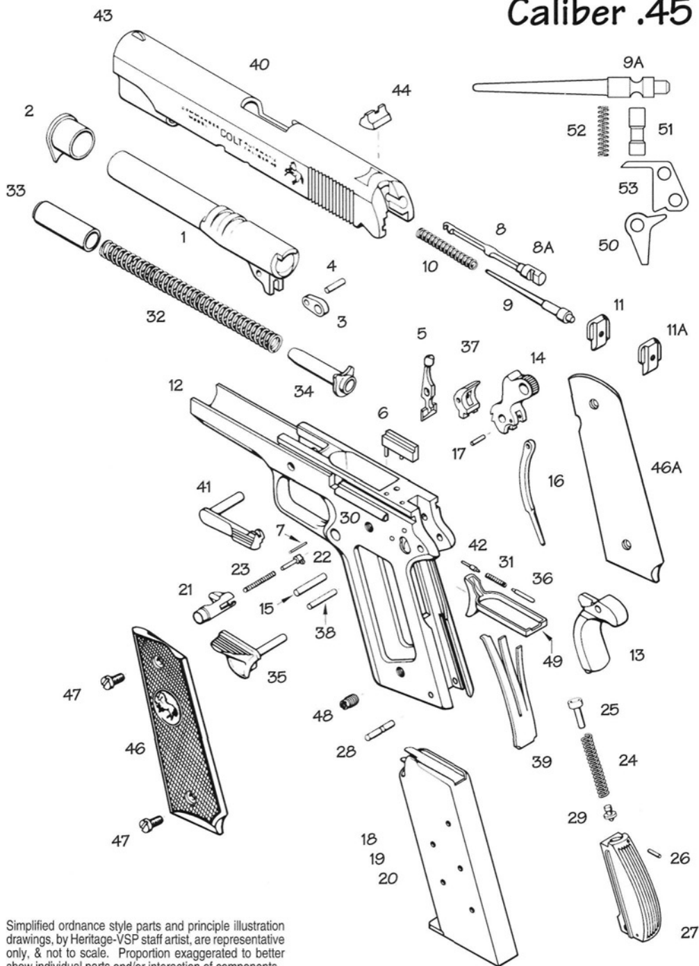
Figure 45- Exploded parts diagram by Heritage - VSP staff artist shows Colt Commander Model and later Series 80 components. Magazine sectional views and components shown in fig. 39. Except for its shorter slide, barrel, bushing, and P-35 style hammer, the Commander is the same as the Government Model. The Commander L. W. Model (aluminum alloy frame) was introduced in 1951. The steel frame Combat Commander was introduced in 1970. Illustration provided as an assembly and parts identification reference.
