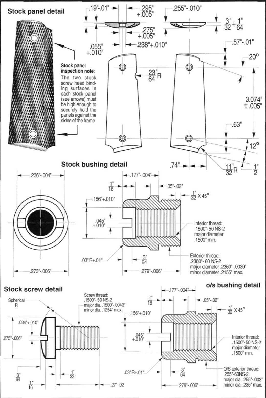
Figure 63- Ordnance style detail drawings by Heritage -VSP staff artist show M1911A1 stock panel, stock screw bushing, oversized stock screw bushing, and stock screw dimensional inspection data. See frame installed component visual and dimensional inspection on page 77 and installation on page 80.
