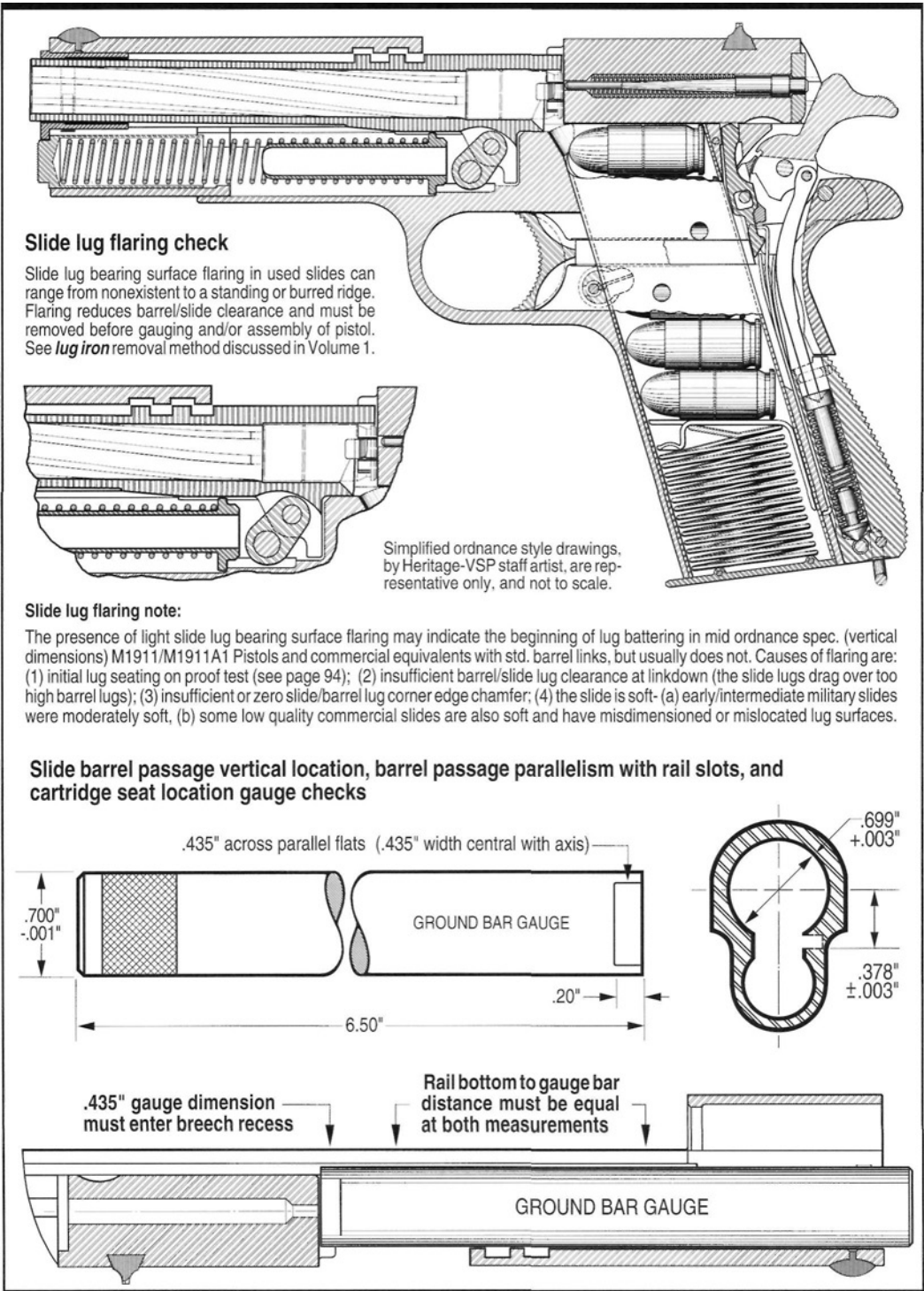
Figure 74- Sectional illustrations, at top, depict insufficient slide/barrel lug clearance at barrel link down. This condition is a known cause of major lug flaring and damage in M1911 pistols. Illustrations, below, show specified location of the slide barrel passage axis above the slide rail slot cuts (specified allowance for nonparallelism of the barrel passage relative to the rail cuts is zero); barrel passage bar gauge dimensional data; and a bar gauge installed in an M1911A1 slide. The two flats on the bar must enter between the slide recoil surfaces (ordnance go gauge - .436"). Determine slide barrel passage parallelism by measuring slide rail bottom to bar gauge top distance at two points with a depth micrometer.
