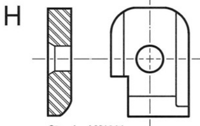
Standard M1911 firing pin stop
