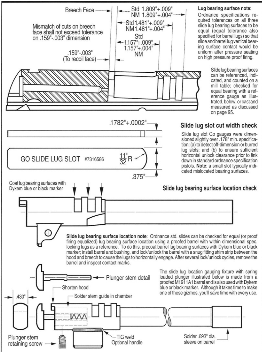
Figure 75- Ordnance style illustration by Heritage -VSP staff artist, at top, shows M1911A1 slide lug bearing surface locations relative to the slide recoil surface and breech face. Lug bearing surface location note: Ordnance specifications required all 3 M1911A1 slide lug slots and bearing surfaces to be machined in one operation with an integral cutter. The logic was that the above 1.157", 1.481" & 1.809" dimensions would all be tolerated exactly the same relative to the slide's recoil surfaces. Commercial M1911 slides with individually cut lug slots may or may not have equally tolerated lug bearing surfaces. Fractionally unequal low/medium heat treat carbon steel slide and barrel lug bearing surfaces will eventually seat and in this way equalize. Unequal slide lugs have been known to stress crack and break medium plus heat treat barrel lugs, notably in high pressure/energy 9mm's. See examples in figure 172.
