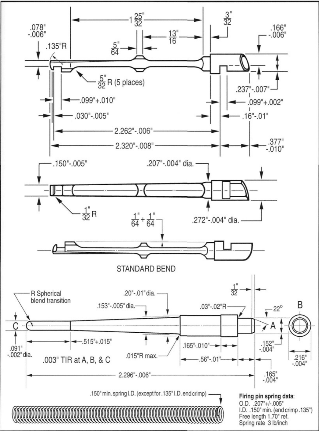
Figure 129- Ordnance style drawings by Heritage - VSP staff artist, show M1911/M1911A1 extractor, firing pin, and firing pin spring dimensional inspection details. Ordnance specified M1911A1 and M1911A1 NM extractor material and heat treat: material- 1060 to 1095 special steel, austenitic grain size 7 or finer; heat treat to RC 48-52. For further data, see ordnance drawing #6008595. Ordnance specified M1911A1 and M1911A1 NM firing pin material and heat treat: material- 1060, 1070, 1095 steel, austenitic grain size 7 or finer; heat treat to A70.5 to 73.5 (C scale equivalent RC 40 - 46). For further data, see ordnance drawing #6008599. Extractor notes: M1911 extractors are basically springs. This being the case, best material is as specified. Regarding commercial products- I would suggest rejecting cast extractors and using well machined, well heat treated extractors made by quality manufacturers, only.
