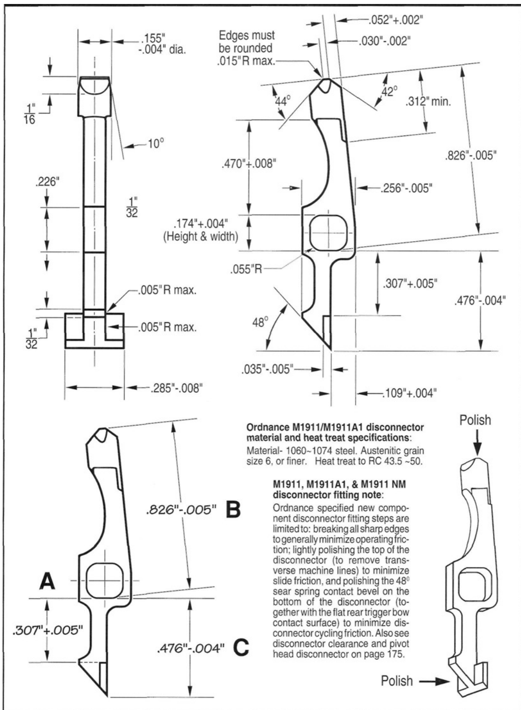
Figure 156- Ordinance style illustrations by Heritage - VSP staff artist show basic M1911/M1911A1 disconnecter dimensional inspection data. For further data, see ordinance drawing #6008603 (disconnecter). Not too many years ago, virtually all M1911/M1911A1 disconnecters sold met ordinance specs. (Those that didn't gauge were rejected.) After visual inspection, it was then sufficient to simply measure overall height. If a disconnecter appeared to be serviceable and measured within 1.293" min. and 1.302" max. OAL, it was considered serviceable. Now, even with benefit of modern CNC equipment, some manufacturers fail to hold tolerances. For this reason, and because safety is involved, all M1911 disconnecters should be dimensionally checked, at least at A, B, and C above, before use.
