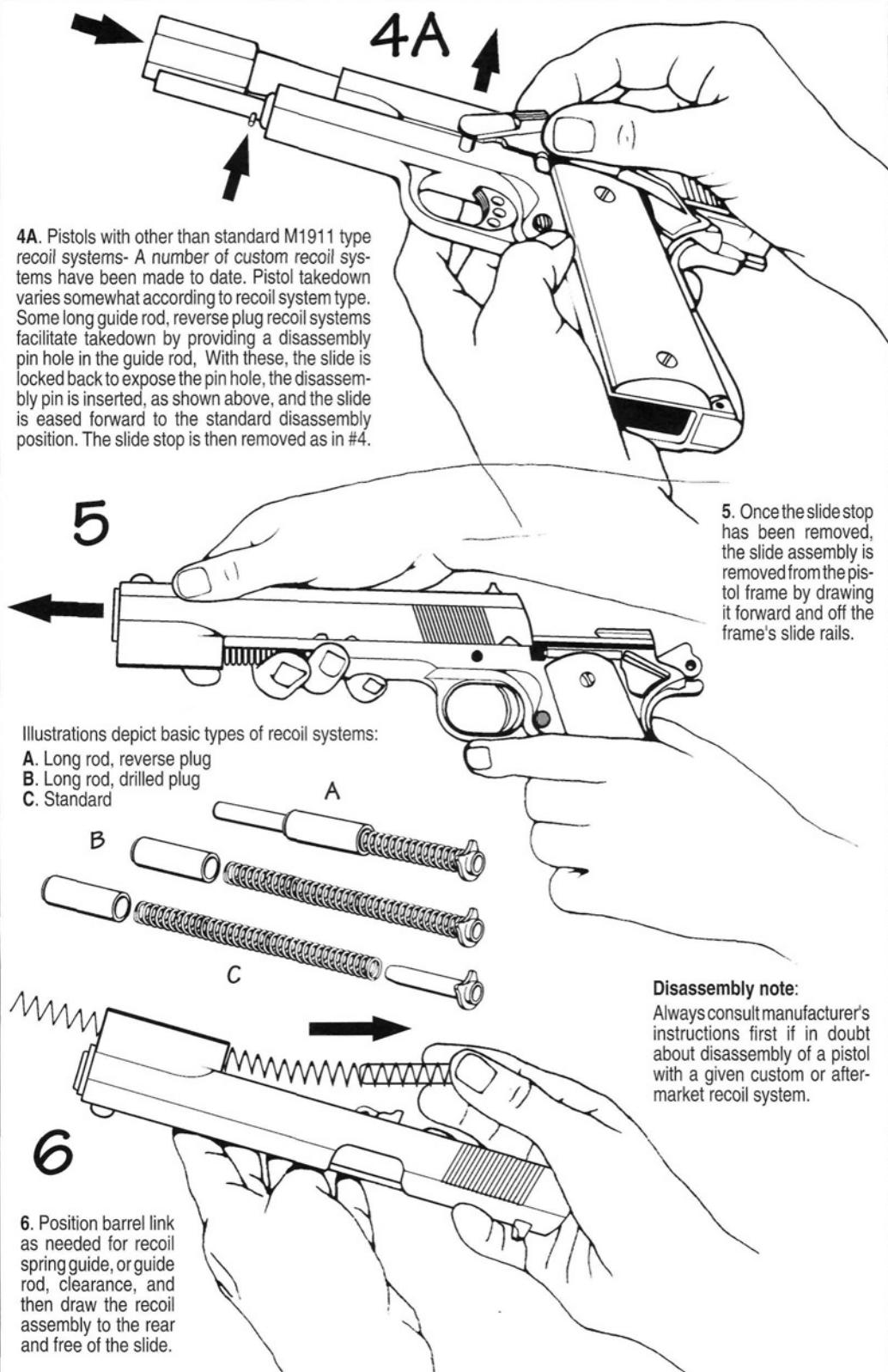
Figure 50- Ordnance style illustrations show M1911/M1911A1 Pistol disassembly steps 4A through 6.
