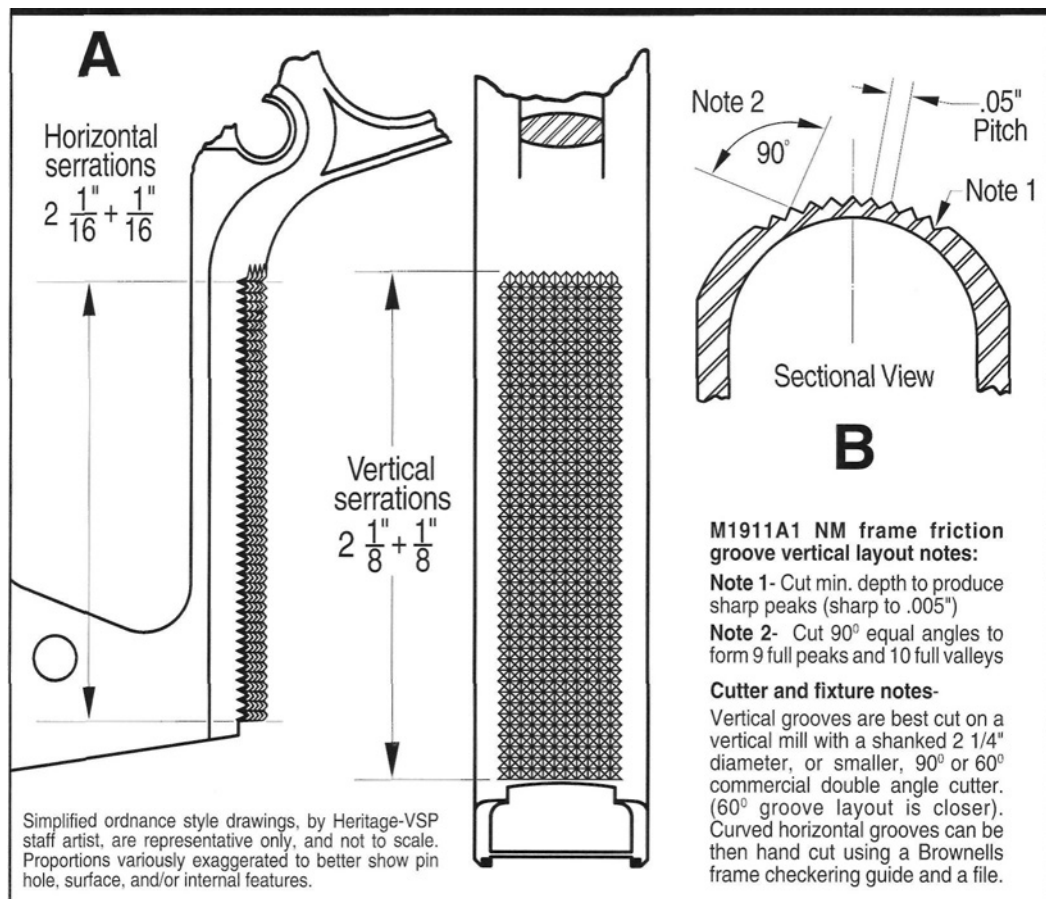
Figure 61- Ordnance style illustrations by Heritage - VSP staff artist, show 90^\circ diamond cut M1911A1 NM style front frame friction groove (frame checkering) modifications at A . Cutting vertical grooves in the frame as shown in the layout, at B , is the first step in cutting the 90^\circ diamond pattern checkering, illustrated at A . Reasonably sharp parallel vertical grooves, although not as stylish in appearance, usually provide sufficient frame grip friction by themselves.
