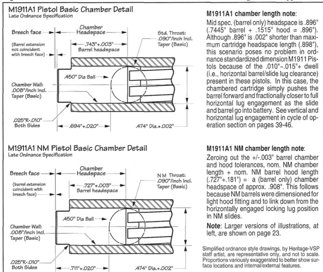
Figure 89- Ordnance style illustrations by Heritage - VSP staff artist show std. M1911A1 and NM barrel chamber and bullet seat dimensional data and barrel (only) chamber length for the M1911 ball cartridge. Keep in mind that std. M1911A1 barrel chamber length is a barrel only headspace reference. Actual chamber headspace is defined as the distance from the chamber's cartridge heading shoulder to the breech face with the barrel in horizontally lug engaged position. In the NM barrel illustrated, the nom. .727" barrel headspace dimension + nom. .181" recoil shoulder to breech face distance would equal a barrel headspace of .908" (.898" NM cartridge length + .010"). Hood fitting would fractionally reduce this figure.
