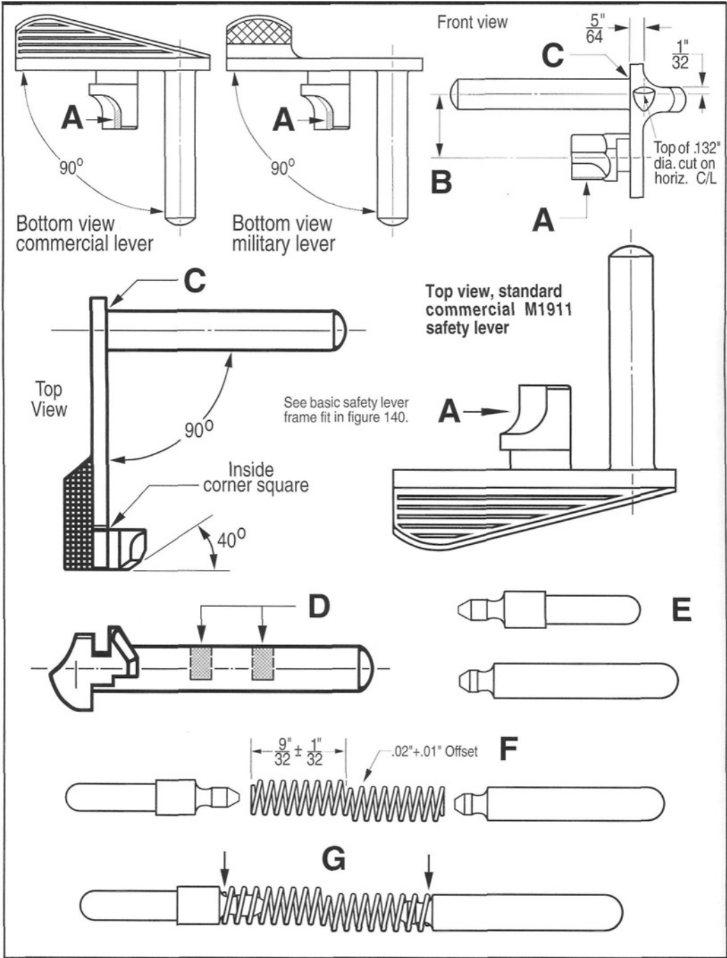
Figure 137- Ordnance style illustrations by Heritage - VSP staff artist show M1911/M1911A1 safety lever, slide stop (slide lock), and safety/slide stop spring and plunger assembly visual inspection points. Critical points are: (1) the safety lever sear stop (sear blocking) surface, at A, must be within ordnance specifications, or long enough to positively block the sear in the pistol the safety is installed in (see sear stop surface fitting on page 169); (2) safety pivot shaft and stop stud axes, at B, must be parallel to minimize angular bind; (3) the inside pin shaft/lever corner radius, at C, must be present on both the safety and the slide stop to minimize stress crack potential; (4) the slide stop crosspin must be checked for lug peening, at D, (shiny lug contact marks should show, only- surface upset indicates the stop is too soft); (5) both plungers, at E, must have smooth spherical ends and serviceable spring inserts; (6) spring offset, at F, must be as shown and spring end crimp(s), at G, must capture both plunger stem spring inserts.
