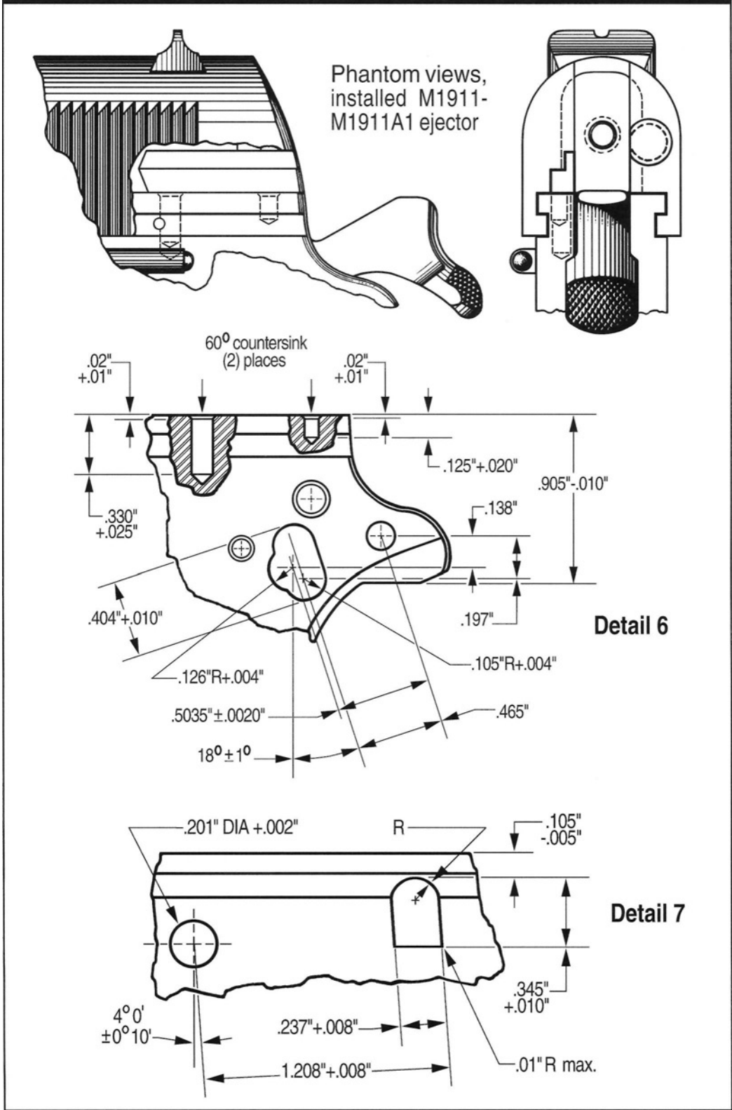
Figure 57- Ordnance style illustrations by Heritage - VSP staff artist, show detail views of critical M1911A1 frame surfaces. Reference numbers are keyed to illustrations on pages 70 and 72.
