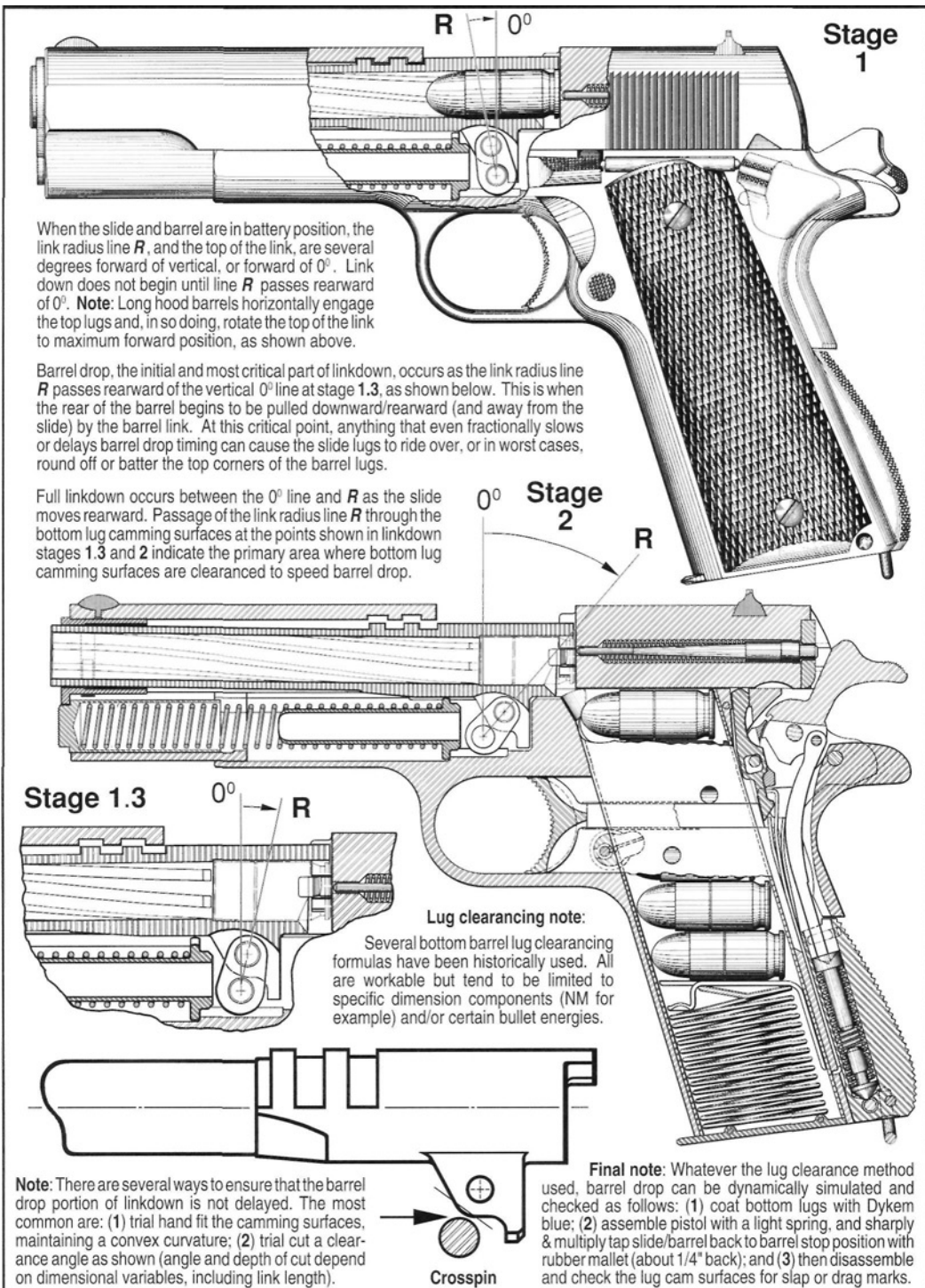
Figure 181- Illustrations depict barrel link down in freeze-framed stages. In stage 1, the link radius line R moves rearward to 0^\circ with initial slide recoil. In stage 1.3, line R passes 0^\circ and unlock and barrel drop occurs. At stage 2, link down ends as the back of the bottom barrel lug comes to rest against the frame's vertical stop surface. Stage 1.3 timing is critical, and doubly so when high energy bullets are fired. A related dynamic link down problem, delayed link down (wherein the barrel is held upward longer than necessary by the bottom barrel lug), most commonly found in tall vertical tolerance stack/long link pistols, is caused by excessive material (relative to link radius length) on the bottom barrel lug camming surfaces.
