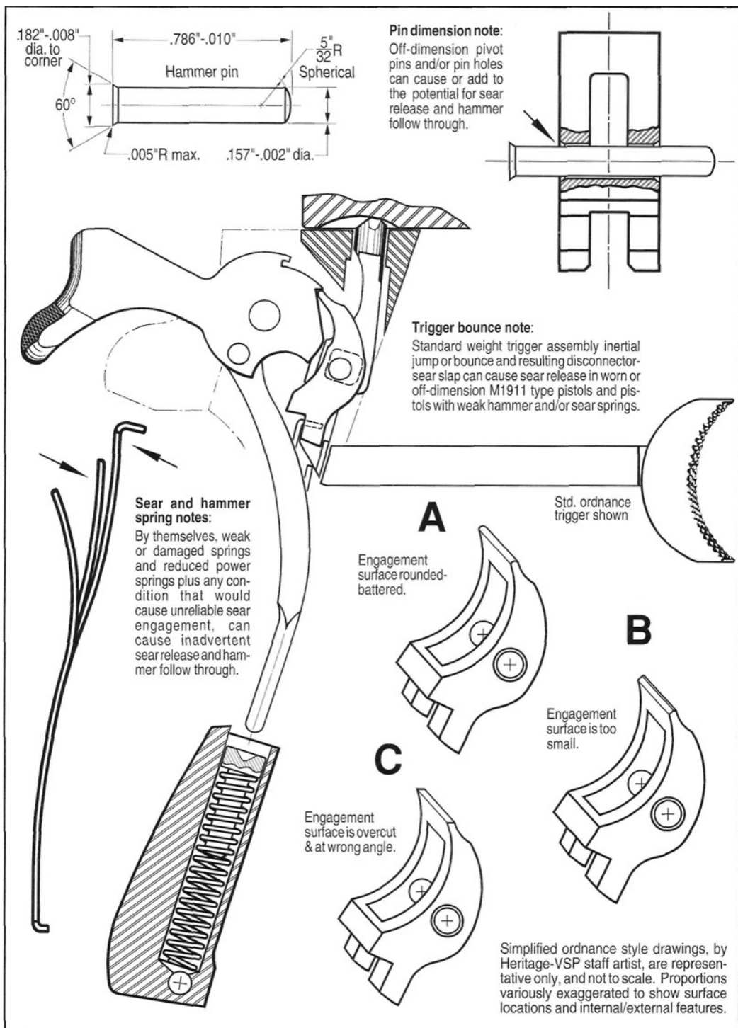
Figure 160- Ordnance style principle illustration by Heritage - VSP staff artist shows factors that can cause and/or contribute to inadvertent sear release and hammer follow through in M1911, M1911A1, and commercial M1911 type pistols. Sear engagement surface conditions that are major causes of, or that predispose, hammer follow through are illustrated above. The sear, at A , has a battered/rounded off engagement; the sear, at B , has a miscut breakaway clearance (almost zero bearing surface area remains); the sear, at C , has a full engagement surface-but, in this example, this surface was cut too short and is nonparallel with sear pin hole axis. See detailed list of interactive causes & potential causes on page 173.
