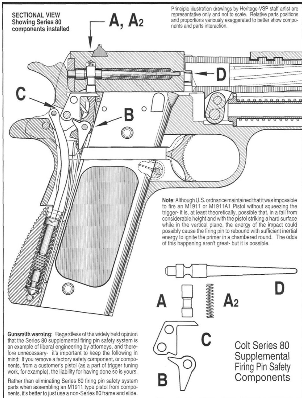
Figure 8- Early ordnance style illustration by VSP - Heritage staff artist, at top, shows relative positions of Colt Series 80 supplemental firing pin safety components in a fully assembled pistol. Series 80 safety components are shown separately, below. The Series 80 firing pin safety system functions as follows: In rest position, the firing pin lock plunger spring (A2) holds the firing pin lock plunger (A) downward and thereby retains (locks) the firing pin (D) in the rearward position. When the hammer is cocked, and the thumb and grip safety are in the ready to fire position, squeezing the trigger (an intentional action) then causes the trigger bow to cycle the trigger bar lever (B), this action, in turn, rotates the firing pin lock plunger lever (C) which elevates the firing pin lock plunger (A) to the firing pin clearance position. This action enables the hammer to impact the firing pin (D) and to move the firing pin forward with sufficient inertial energy to initiate the primer in a chambered round.
