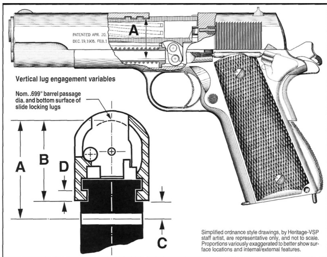
Figure 81- Ordnance style phantom and sectional illustrations, by Heritage - VSP staff artist, show internal operating surface locations in an M1911A1 Pistol referenced from the center of the slide stop crosspin hole in the frame and from the bottom of the slide rails. Critical vertical tolerance stack dimensions referenced above are listed and discussed below. Barrels link up higher on a given link radius in pistols with lower aggregate vertical tolerance stack dimensions. For this reason, frames and slides to be used in assembling improved performance and competition M1911 pistols should be preselected by measurement (cherry picked) for closest to mid tolerance spec, dimensions.
