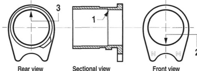
Figure 100- Ordinance style illustrations by Heritage - VSP staff artist show M1911/M1911A1 and NM barrel bushing fitting and clearance data- also applicable to commercial M1911's with similar bushings.
