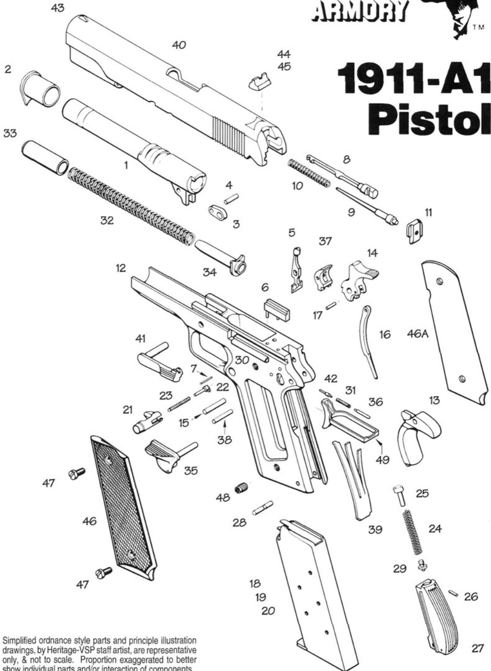
Figure 47- Exploded parts diagram by Heritage -VSP staff artist shows Springfield, Inc. M1911-A1 Pistol components. .45 ACP magazine sectional views in fig. 39 and parts nomenclature on page 50 also apply. M1911-A1 parts illustration is provided as an assembly/disassembly and parts identification reference.
