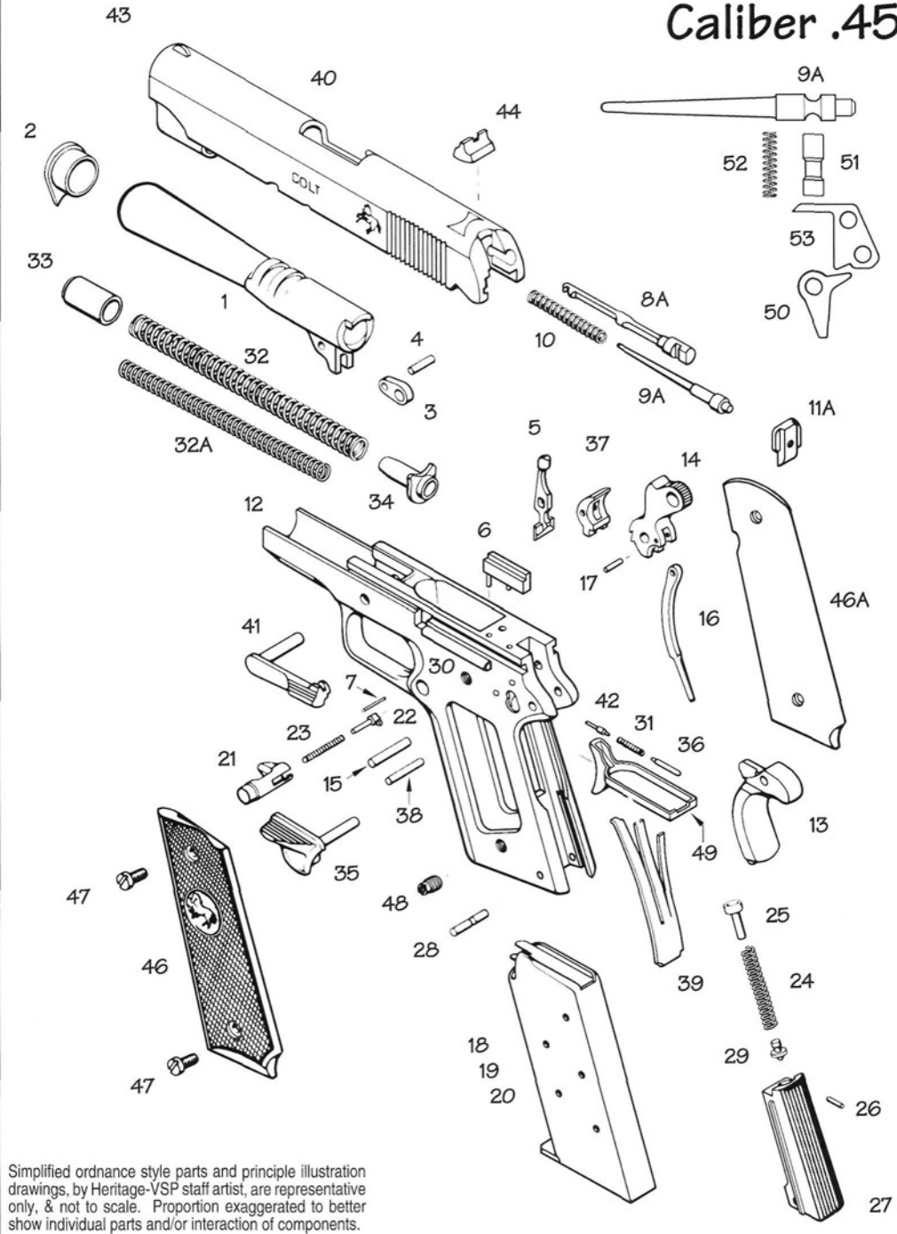
Figure 46- Exploded parts diagram by Heritage - VSP staff artist shows Colt Officer's ACP Model components. This model (introduced 1984) followed the ultra short/reduced height concealed carry pistols pioneered by Detonics and others. The Colt brand name and the practical size of the Officer's ACP served to popularize the extra short M1911 variants. Major differences, other than smaller dimensions, include: a conical barrel and bushing and a redesigned recoil system (2 recoil springs, a short follower, and a reverse plug with lock detent). Illustration provided as an assembly & parts identification reference.
