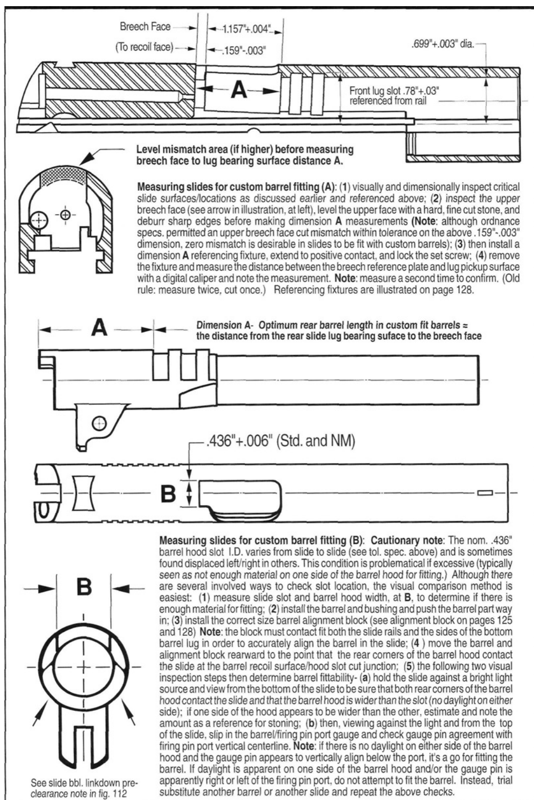
Figure 113- Sectional and exterior view illustrations by Heritage - VSP staff artist, show slide and barrel areas measured in preparation for custom barrel fitting. Measuring/gauging fixtures are shown on page 128. Barrel fitting steps are discussed on pages 125 and 126.
