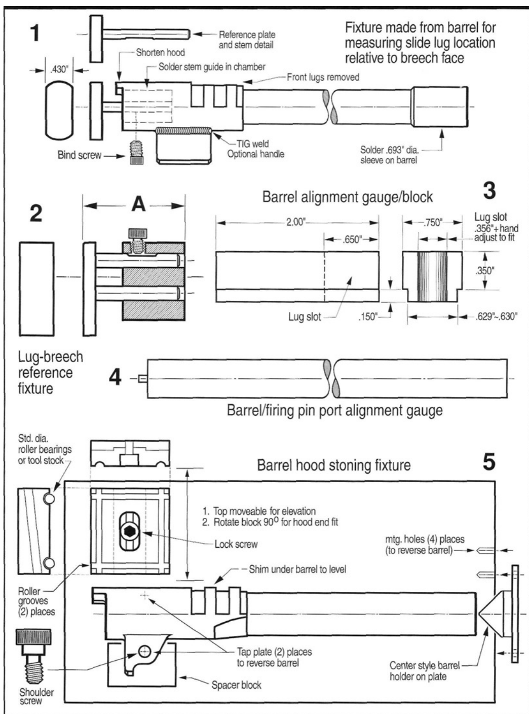
Figure 114- Illustrations show optional fixtures/gauges used to accurately fit custom M1911 barrels. The dimension A reference fixture, at 1, is easily made from an old barrel with serviceable lugs. The reference fixture, at 2, is a design variant by Badger Ordnance. Both are measured with a digital caliper after adjusting to #1 slide lug contact. The Cherry Corners barrel alignment block, illustrated at 3, is available from Brownells, Inc. Barrel alignment blocks can be used as barrel hood fitting guides and also as barrel/slide alignment Go-No Go gauges. Note: Because of slide and barrel lug dimensional variations, blocks are needed in several adjusted sizes. The Brownells barrel/firing pin port gauge, at 4, is a necessary inspection and final fitting reference as discussed earlier. The adjustable barrel hood stoning fixture, designed by author and illustrated at 5, permits precise, flat, and level stoning of barrel hood fitting surfaces.
