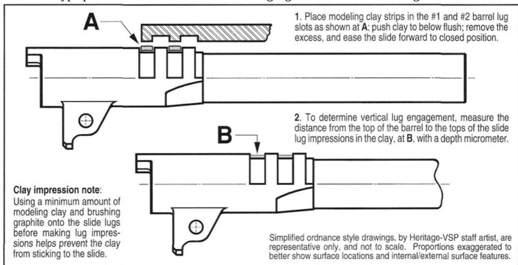
Figure 107- Ordnance style illustrations by Heritage - VSP staff artist show the basic clay strip lug impression method used to determine barrel locking lug vertical engagement in ordnance std. M1911, M1911A1, and commercial equivalent pistols. See clay impression note, above.
