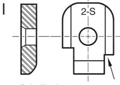
Series 80 variant (notched for plunger lever)
