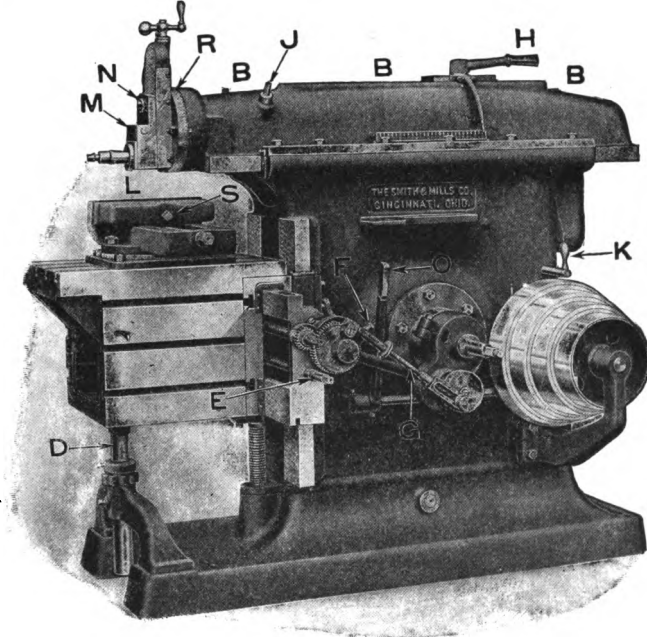
FIG. 13. TWENTY-INCH SHAPER
