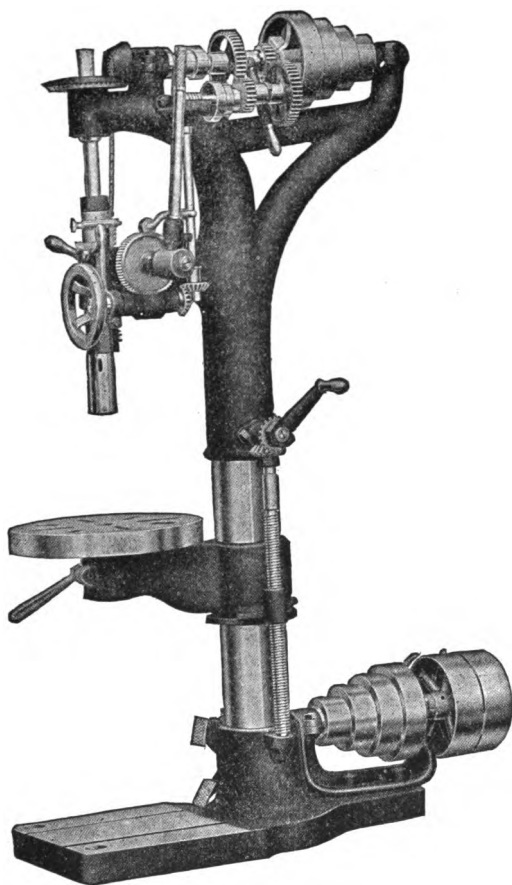
FIG. 31 TWENTY-INCH COMPLETE DRILL
